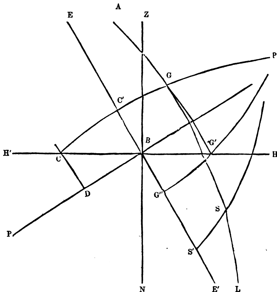
A rule for calculating the time of the heliacal rising of Agastya (Canopus) in a given latitude. In order to explain its rationale, we at first apply the longitude and latitude of Agastya given in the modern Sūrya Sidhānta, viz. 90° longit. and 80° southern latit. Let H H' be the horizon, P the pole of the
